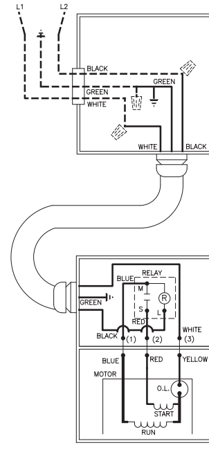
WIRING DIAGRAM FOR MODELS "N3137" All Revisions and "E3137" All Revisions 10/87 (WT) thru Current
